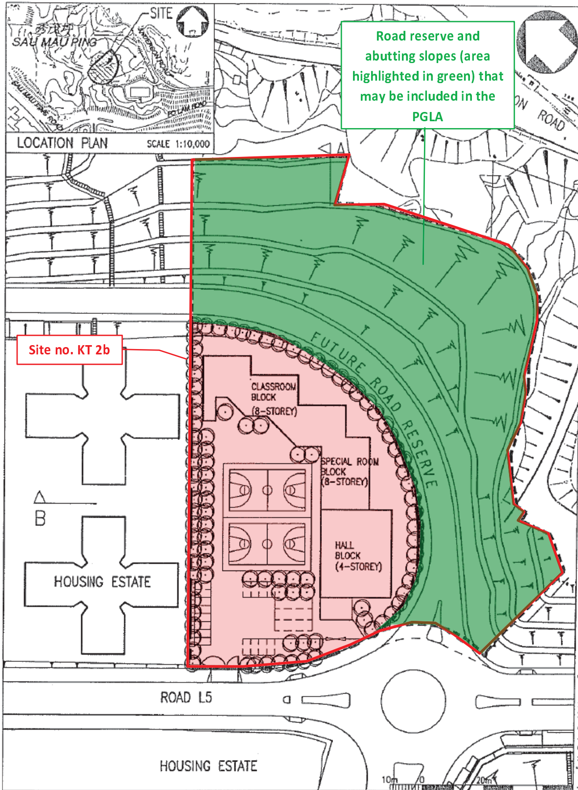
Site Plan – Development at Anderson Road, Kwun Tong, Kowloon (Site no. KT 2b)
