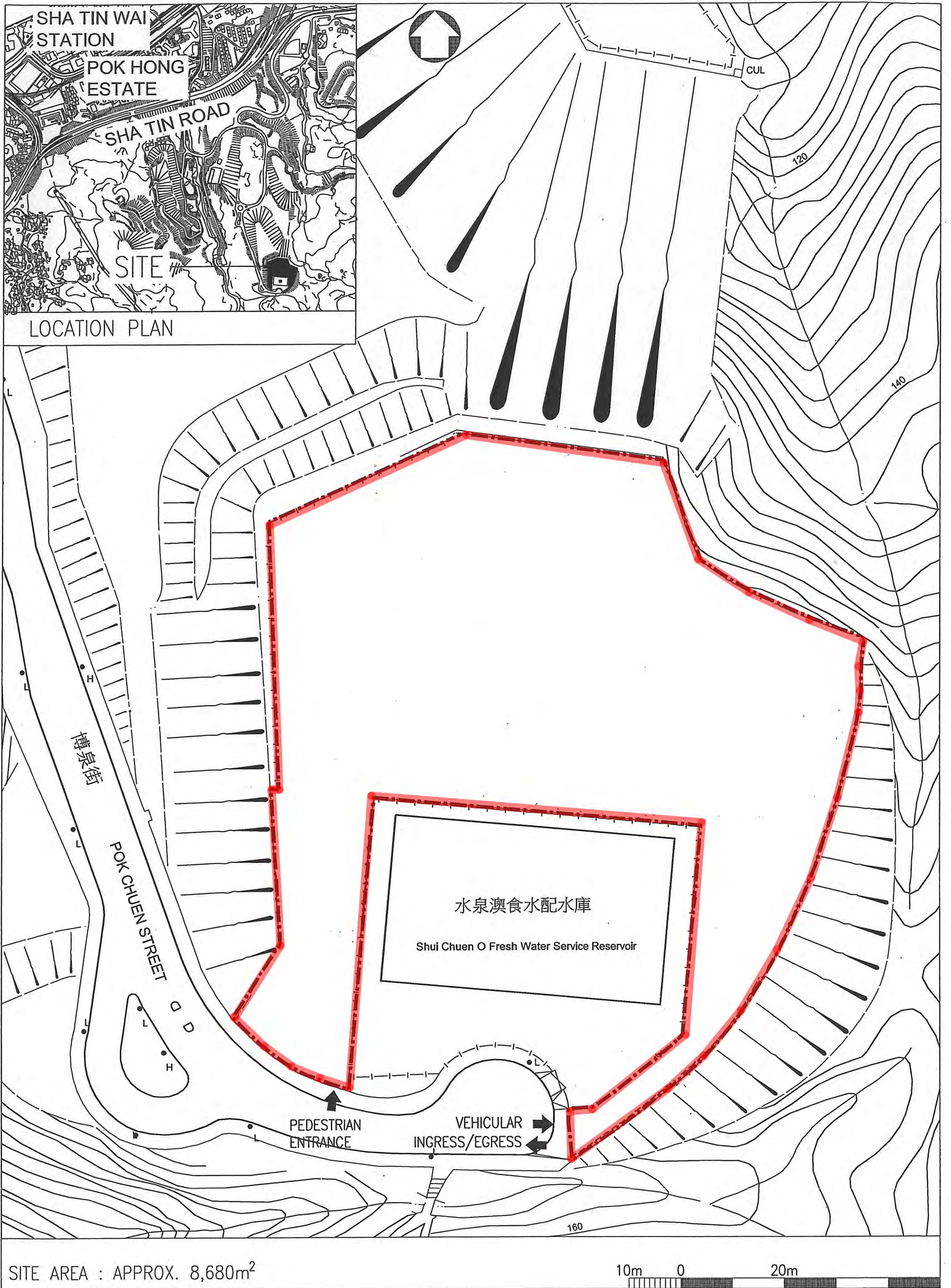
Site Plan - A 30-classroom Primary School at Shui Chuen O, Sha Tin
