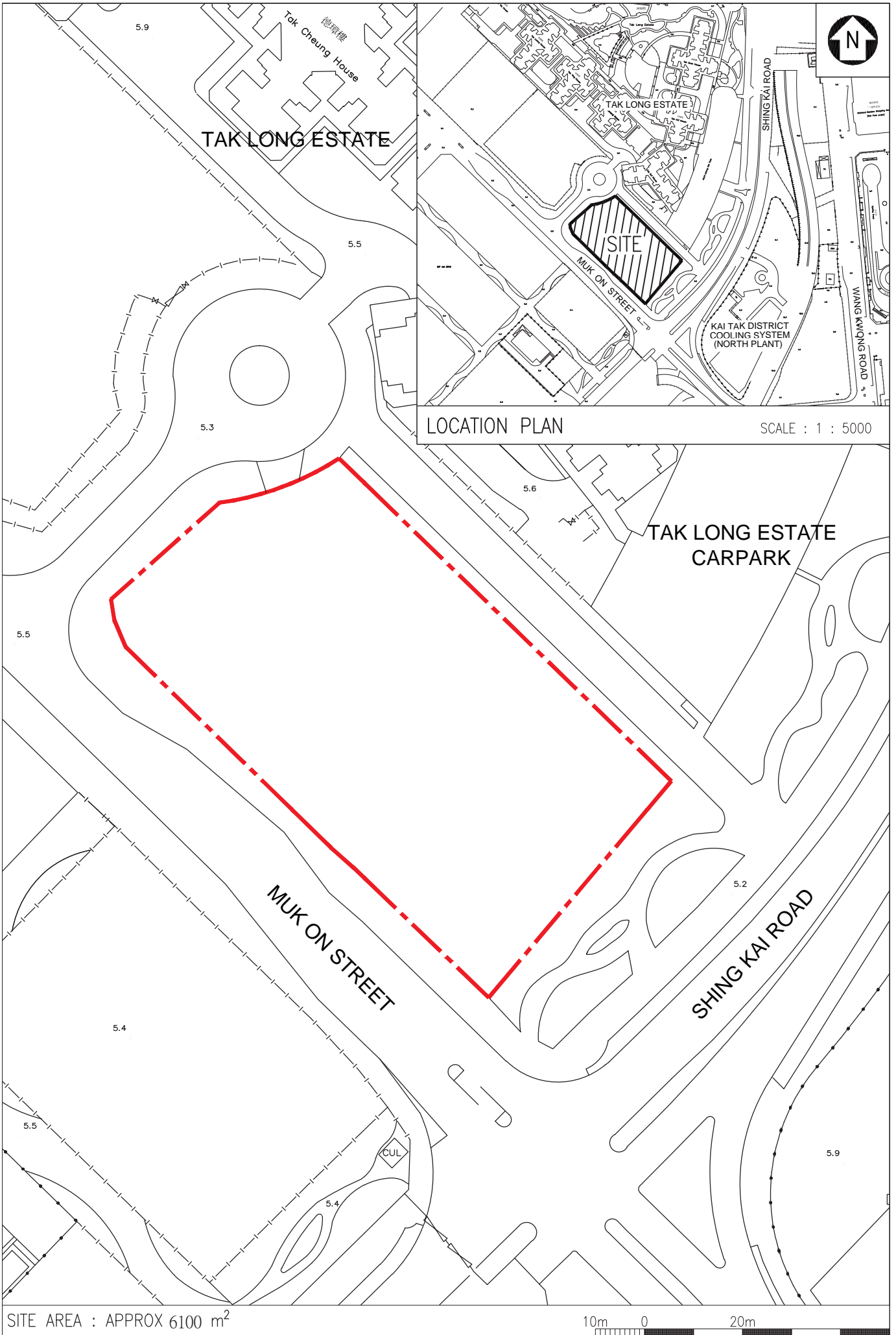
LOCATION PLAN - A 30-CLASSROOM PRIMARY SCHOOL AT SITE 1B-4, KAI TAK DEVELOPMENT
