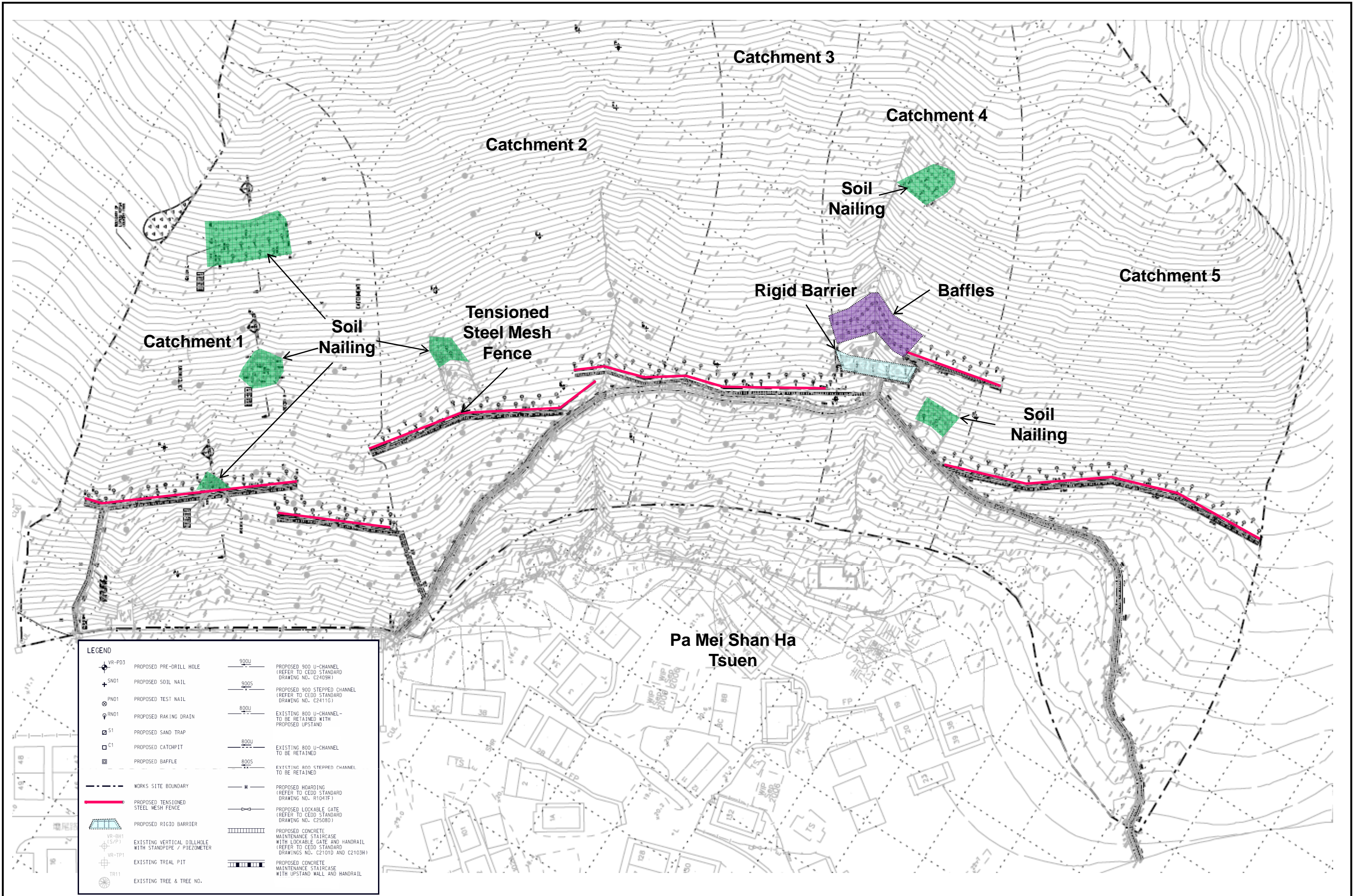
Figure 2 – Proposed Mitigation Works at Pa Mei Site
